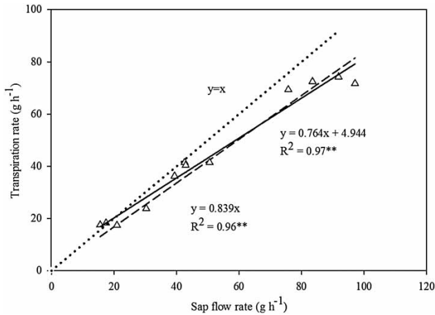
Figure 3 | Compared measured weight loss on a balance with the corresponding sap flow rate calculated according to the sap flow gauge of potted maize; statistical significance level is at p < 0.01 .
